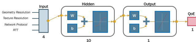
Fig. 6. The neural network architecture used for predicting the QoE of the TI system used in this survey. The numbers below the neural networks components denote the amount of input parameters, hidden and output cells used to predict the final QoE value.
